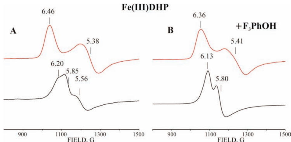
Figure 8. Low-field X-band EPR spectra of cryogenerated (red) and resting high-spin ferric forms (black) of DHP in the absence of substrate (A) and in the presence of 50 mM F_3PhOH in 20% glycerol/0.1 M potassium phosphate buffer, pH 7. Conditions: T = 8 K; modulation amplitude, 10 G; microwave power, 10 mW; microwave frequency, 9.38 GHz.
