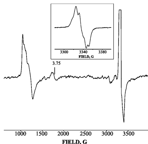
Figure 4. EPR spectra of intermediates arising during the reaction between 0.5 mM ferric DHP and 2.5 mM H_2O_2 in 0.05 M Tris buffer, pH 9, rapid freeze-quenched in 15 ms. Inset: EPR spectrum of radical species arising during this reaction. Conditions: T = 8 K; microwave power, 10 mW; modulation amplitude, 10 G; microwave frequency, 9.38 GHz. Inset: T = 25 K; microwave power, 0.1 mW; modulation amplitude, 3 G.
