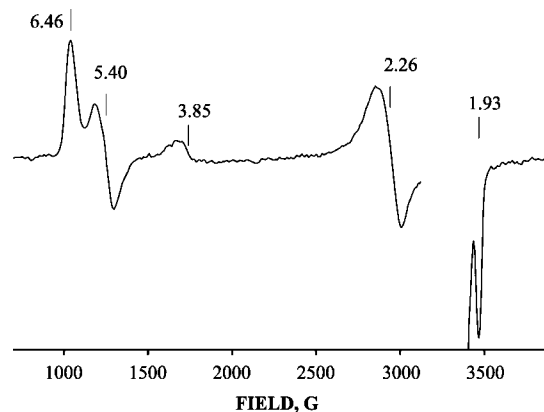
Figure 7. EPR spectrum of 1 mM ferrous DHP in 15% glycerol/0.1 M potassium phosphate buffer, pH 7, exposed to \gamma -irradiation (dose of 1.9 Mr) at 77 K. Conditions: T = 14 K; microwave power, 2 mW; modulation amplitude, 10 G; microwave frequency, 9.382 GHz.
