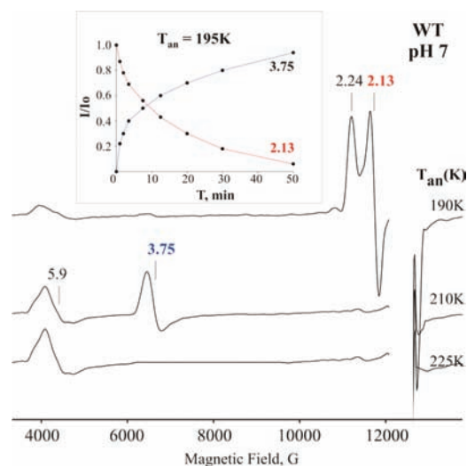
Figure 3. Q-band EPR spectra at 2 K of cryoreduced oxyferrous DHP in 16% glycerol/0.1 M potassium phosphate buffer, pH 7, after stepwise annealing at 190–225 K for 1 min. Inset: kinetic decay of peroxoferric DHP intermediate ( g_1 = 2.24 species) measured at g_2 = 2.13 and growth of g = 3.75 intermediate at 195 K. Conditions: T = 2 K; microwave power, 20 \mu W; modulation amplitude, 1 G; microwave frequency, 34.99 GHz.
