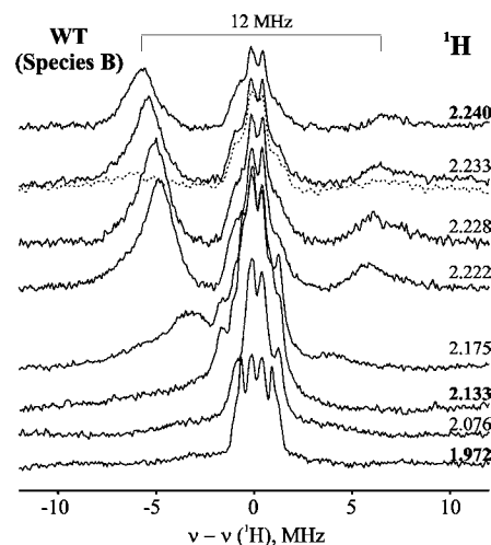
Figure 6. 2D frequency/field ^1\text{H} CW ENDOR spectra of cryoreduced oxyferrous DHP in 16% glycerol– \text{H}_2\text{O}/0.1 M potassium phosphate buffer, pH 7, annealed at 189 K for 1 min (the B species, solid line) and in d_3 -glycerol– \text{D}_2\text{O}/0.1 M potassium phosphate buffer, pH 6.6 (dashed line). Conditions are the same as described in Figure 5.
