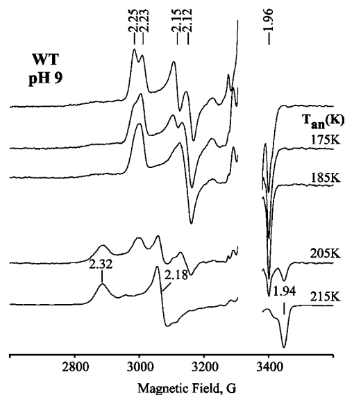
Figure 2. EPR spectra of cryoreduced oxyferrous wild-type DHP in 16% glycerol/0.05 M Tris buffer, pH 9, annealed at indicated temperatures. Conditions: T = 25 K; microwave power, 10 mW; modulation amplitude, 5 G; microwave frequency, 9.38 GHz.
