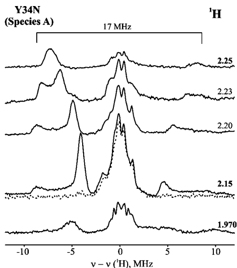
Figure 5. 2D frequency/field ^1\text{H} ENDOR spectra of cryoreduced oxyferrous Y34N DHP in 16% glycerol– \text{H}_2\text{O}/0.1 M potassium phosphate buffer, pH 7 (species A, solid line) and in d_3 -glycerol– \text{D}_2\text{O}/0.1 M potassium phosphate buffer, pH 6.6 (dotted line). Conditions: T = 2 K; microwave frequency, 34.99 MHz; modulation amplitude, 2 G; scan rate, 0.5 MHz/s; rf power, 7 W; frequency bandwidth, 60 kHz.
